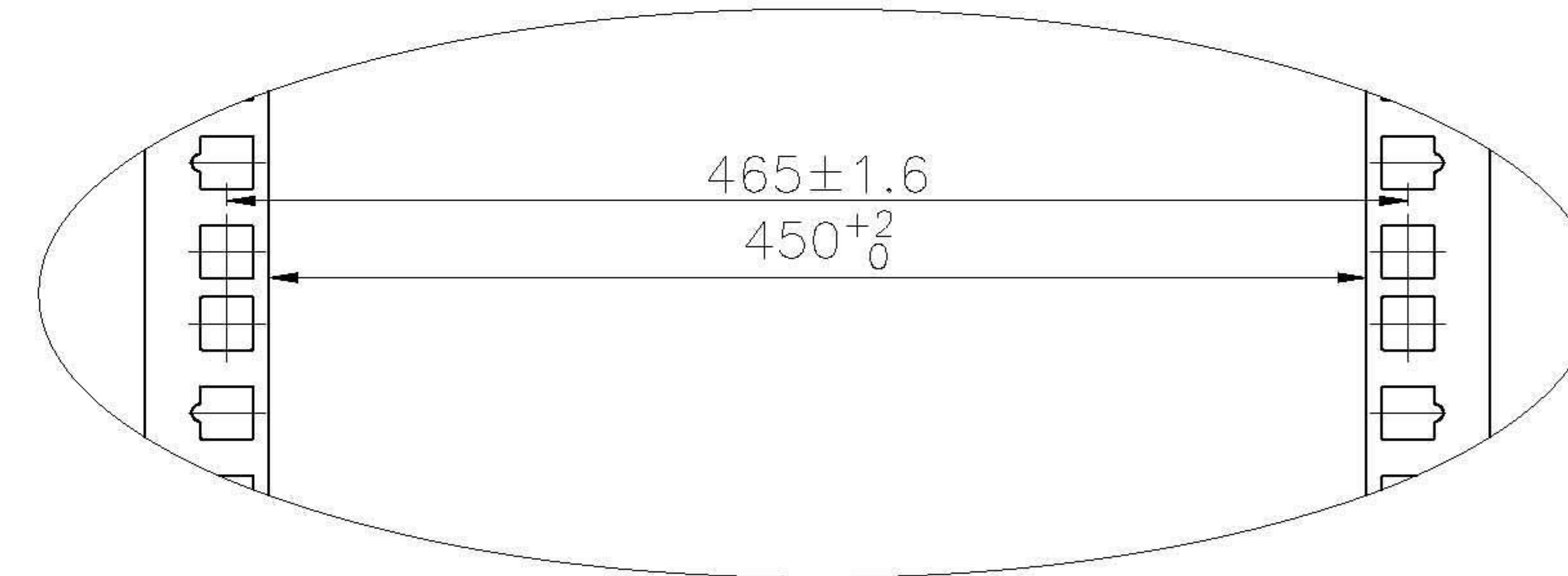
Installation dimension for mounting profile
