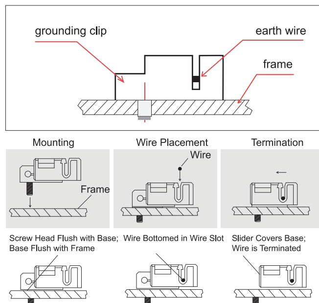
Figure 6: Installation Methods
